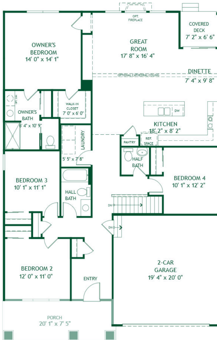
CRAFTSMAN FIRST FLOOR - BASE PLAN
